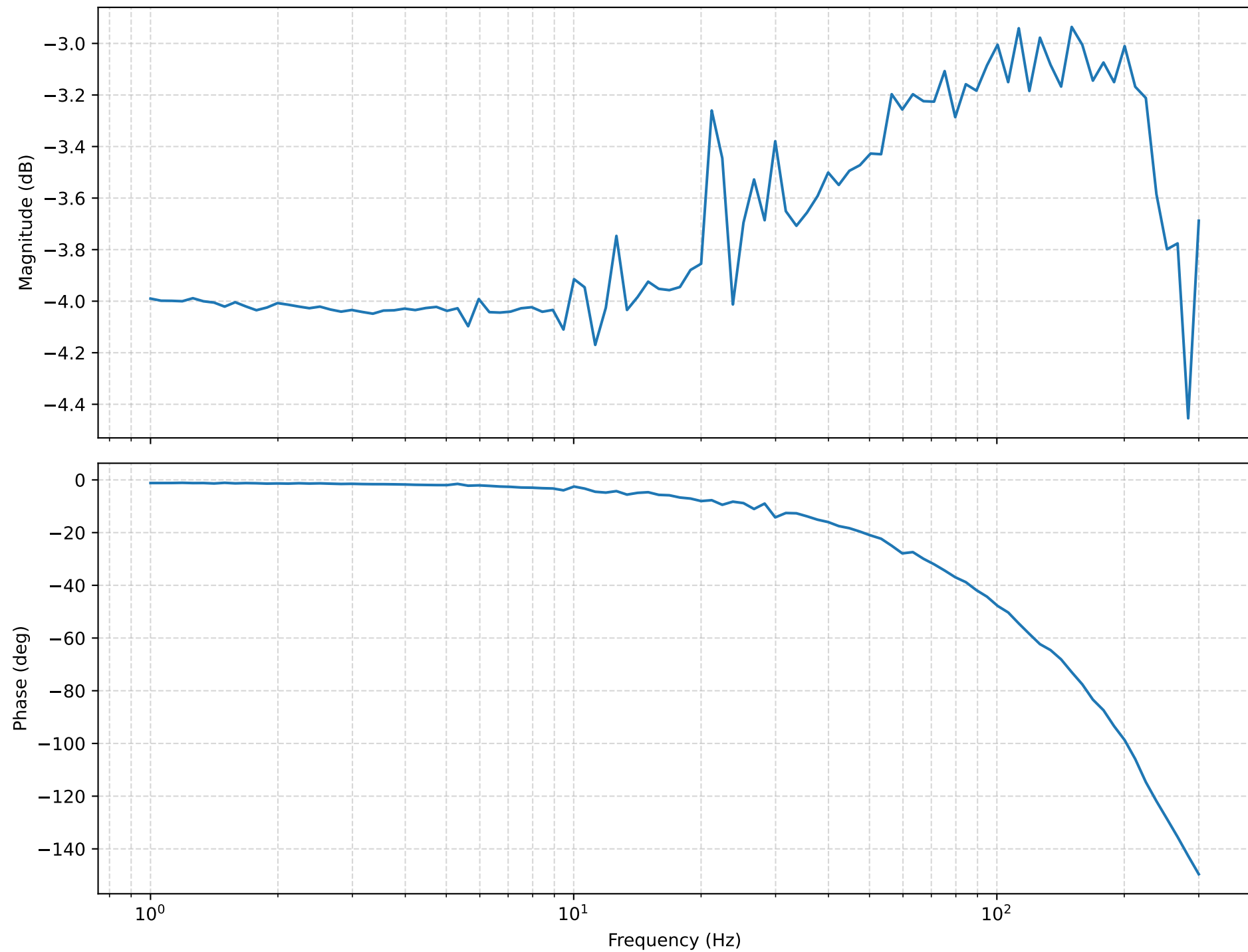
Bode Plot
